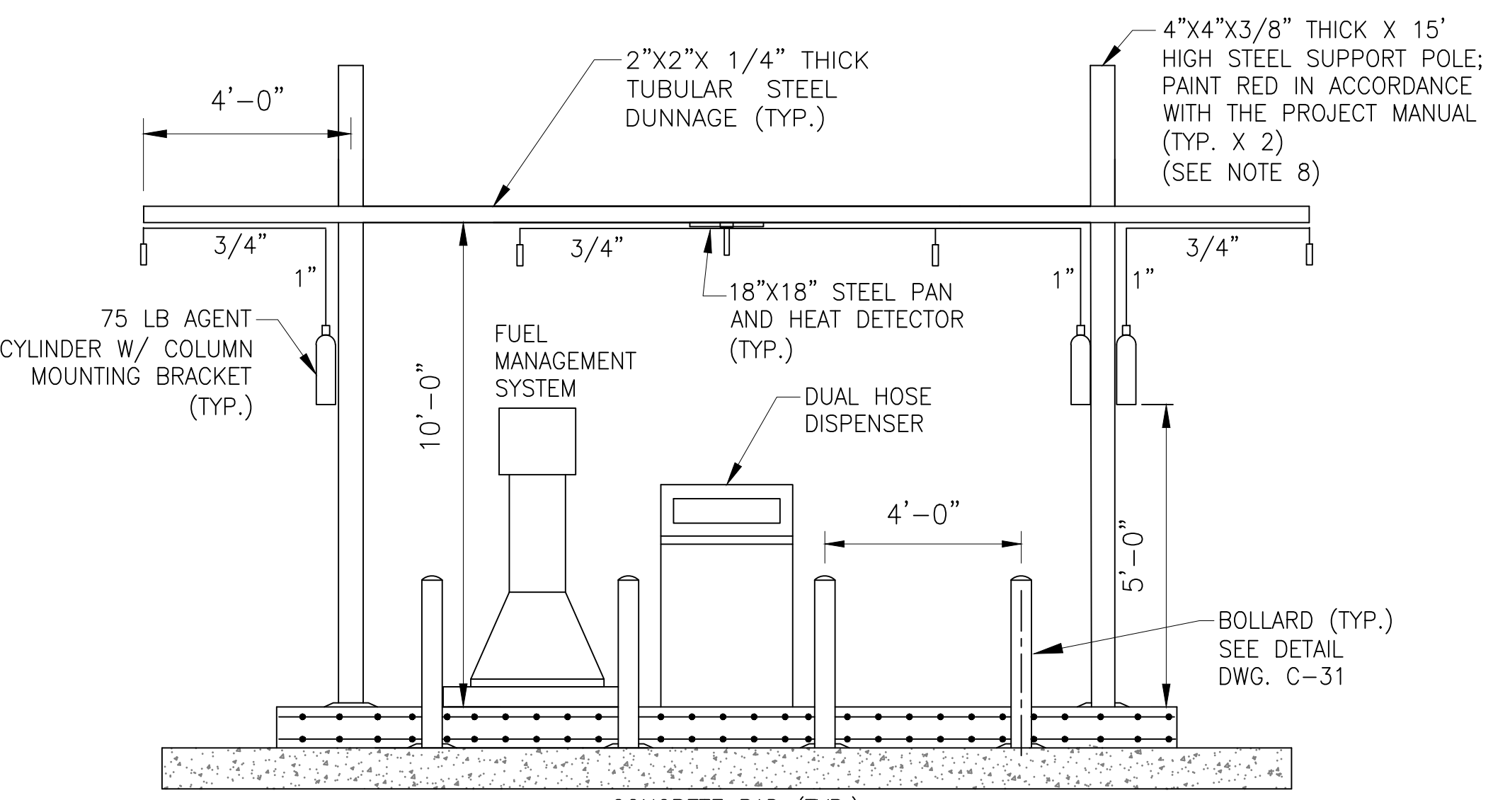
DUAL HOSE DISPENSER ISLAND ELEVATION
