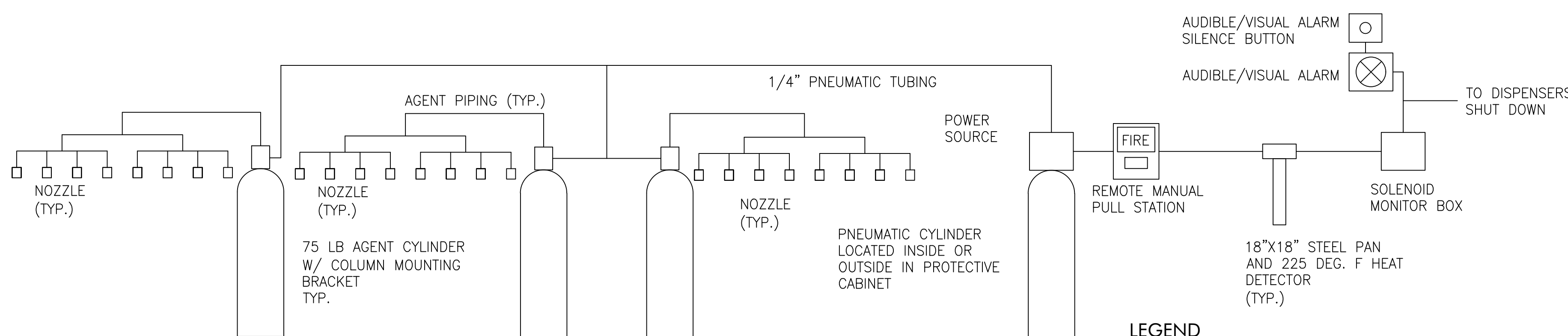
FIRE SUPPRESSION SCHEMATIC DIAGRAM
